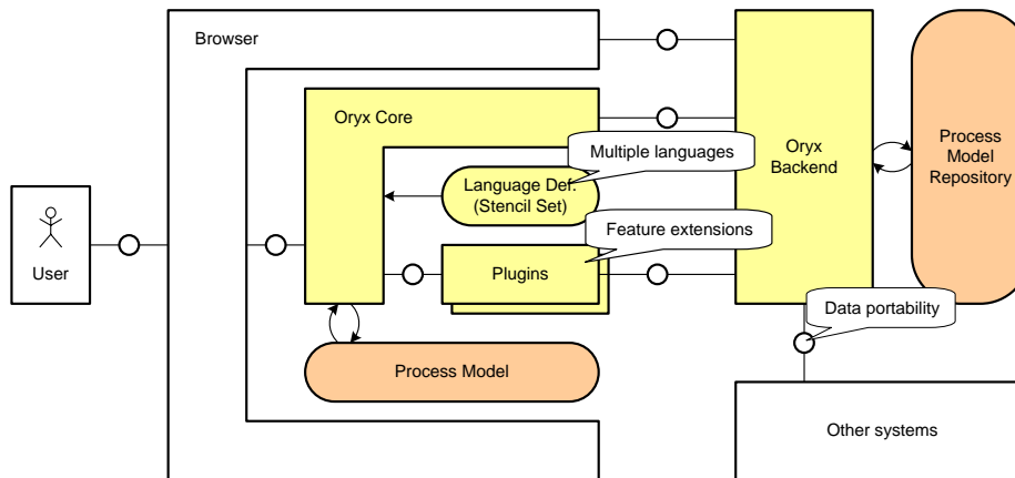
Fig. 1. Oryx architecture
