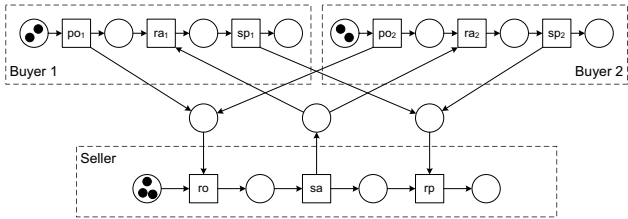
Figure 3. Concurrent conversations
