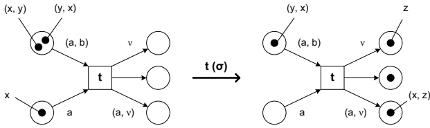
Figure 4. Sample \nu^* -net and firing of t
