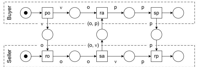
Figure 5. Interconnection model N
