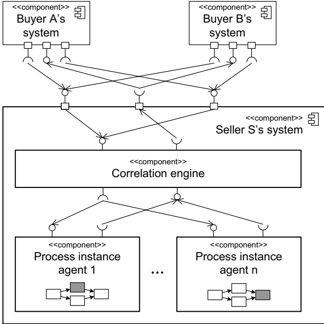
Figure 1. Architectural overview: Correlation engine and process instance agents
