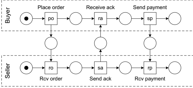
Figure 2. Classical place/transition net
