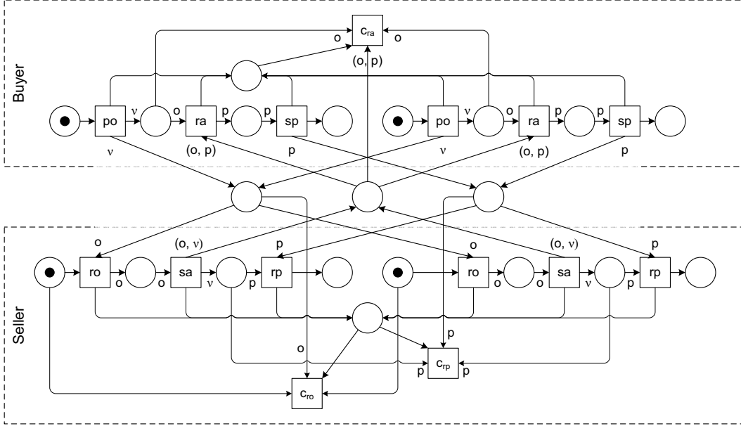
Figure 7. Addition of competition transitions
