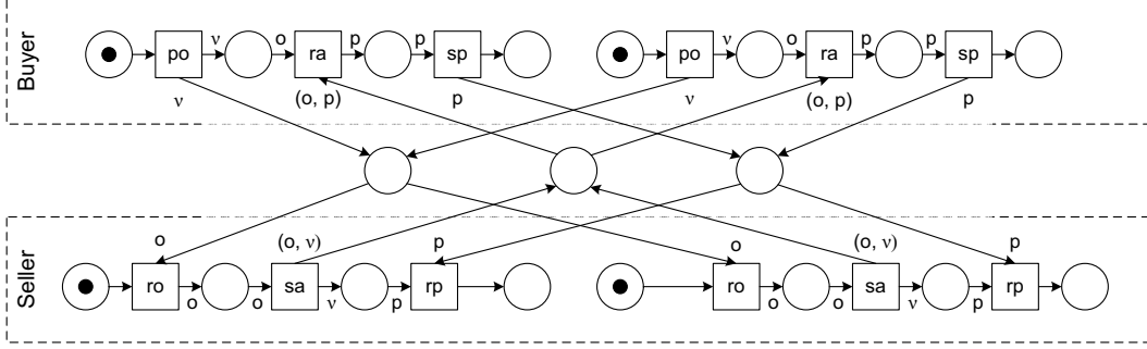
Figure 6. Representing two concurrent conversations
